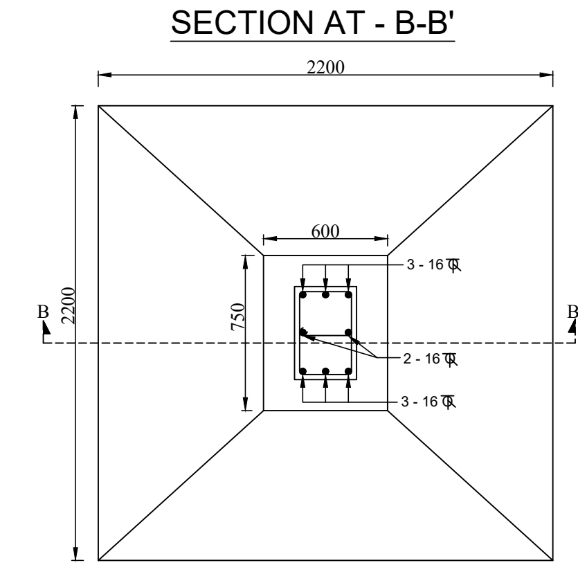
DETAILS OF R.C.C FOOTING (F2) TYP. SCALE-1:25
