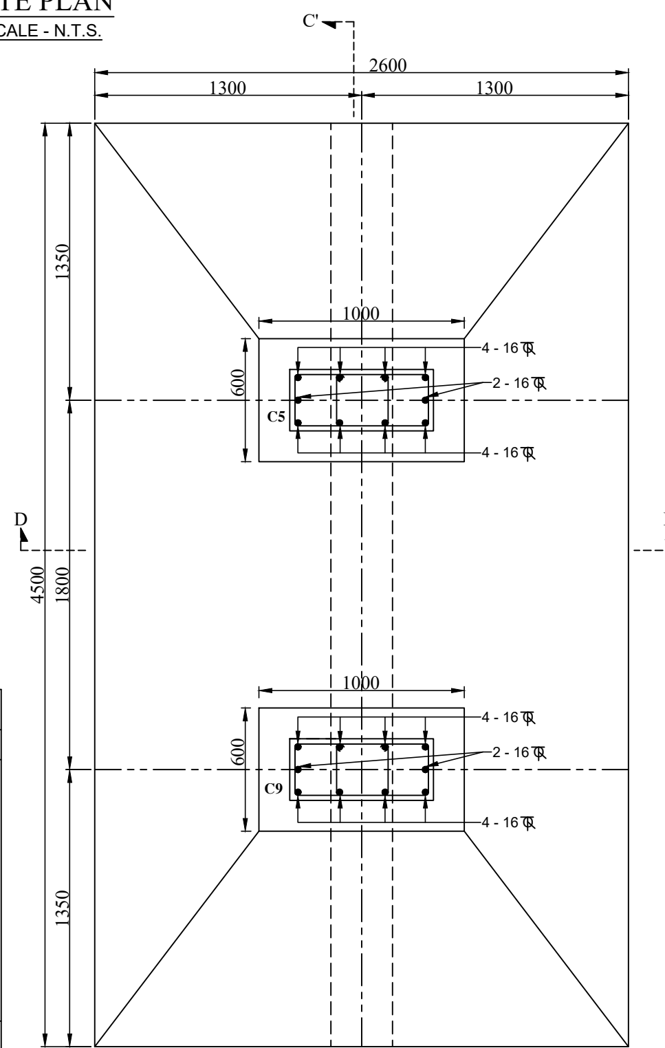
DETAILS OF R.C.C FOOTING (F3) TYP. NOTES :- SCALE-1:25
