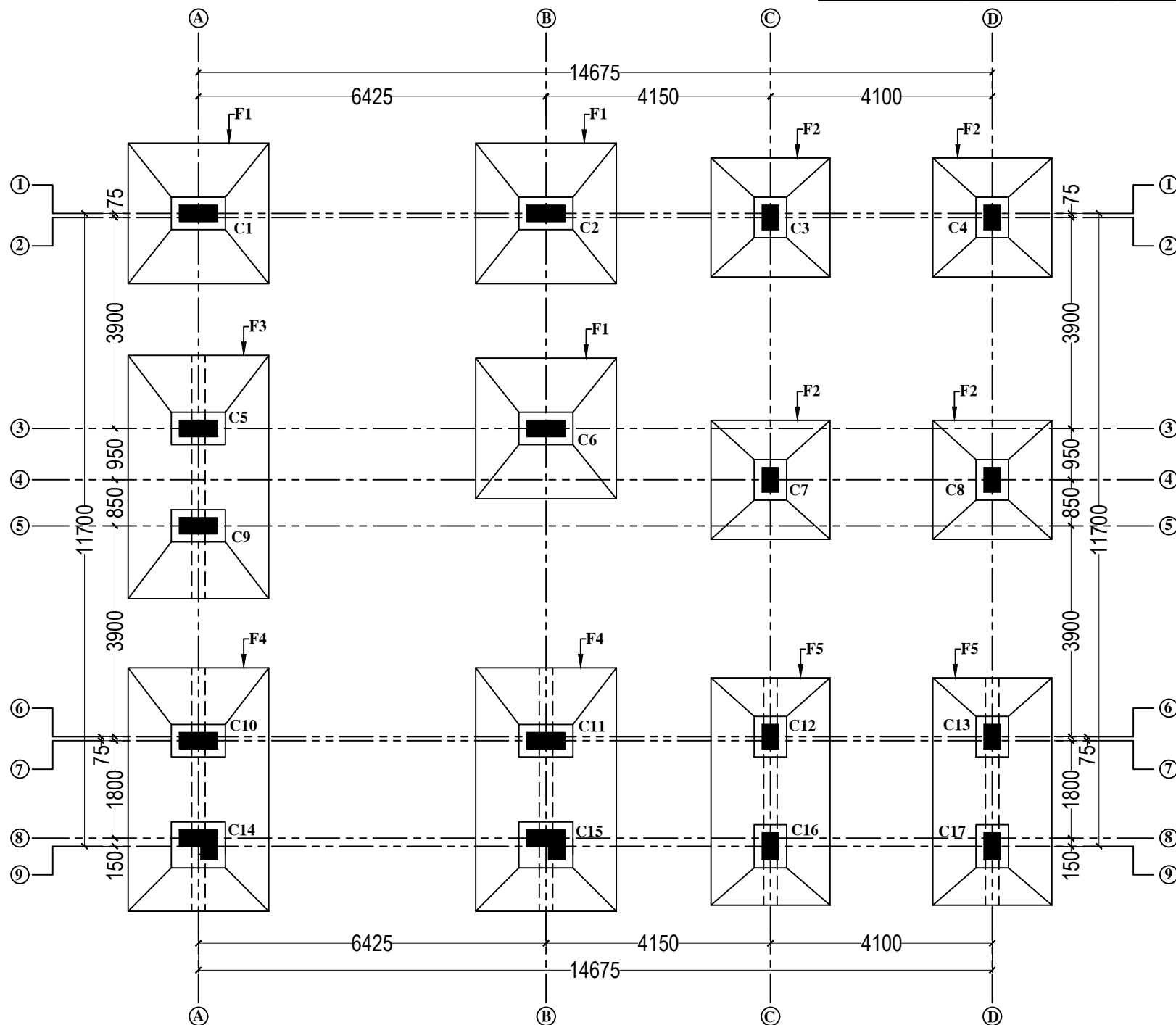
COLUMN & FOUNDATION LAYOUT PLAN
