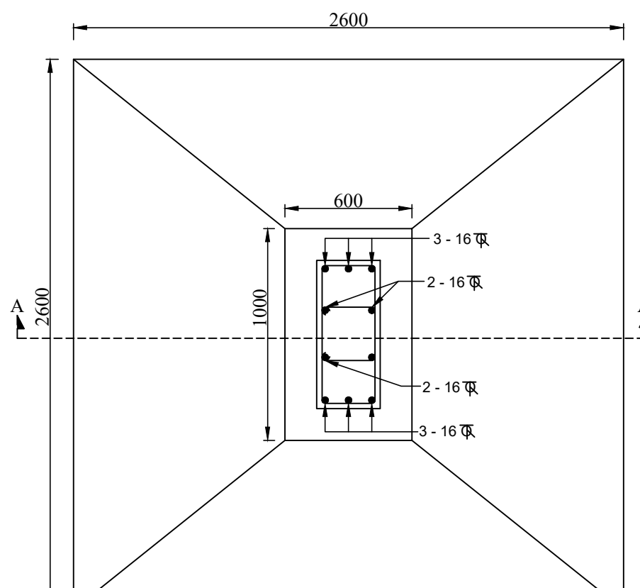
DETAILS OF R.C.C FOOTING (F1) TYP.
