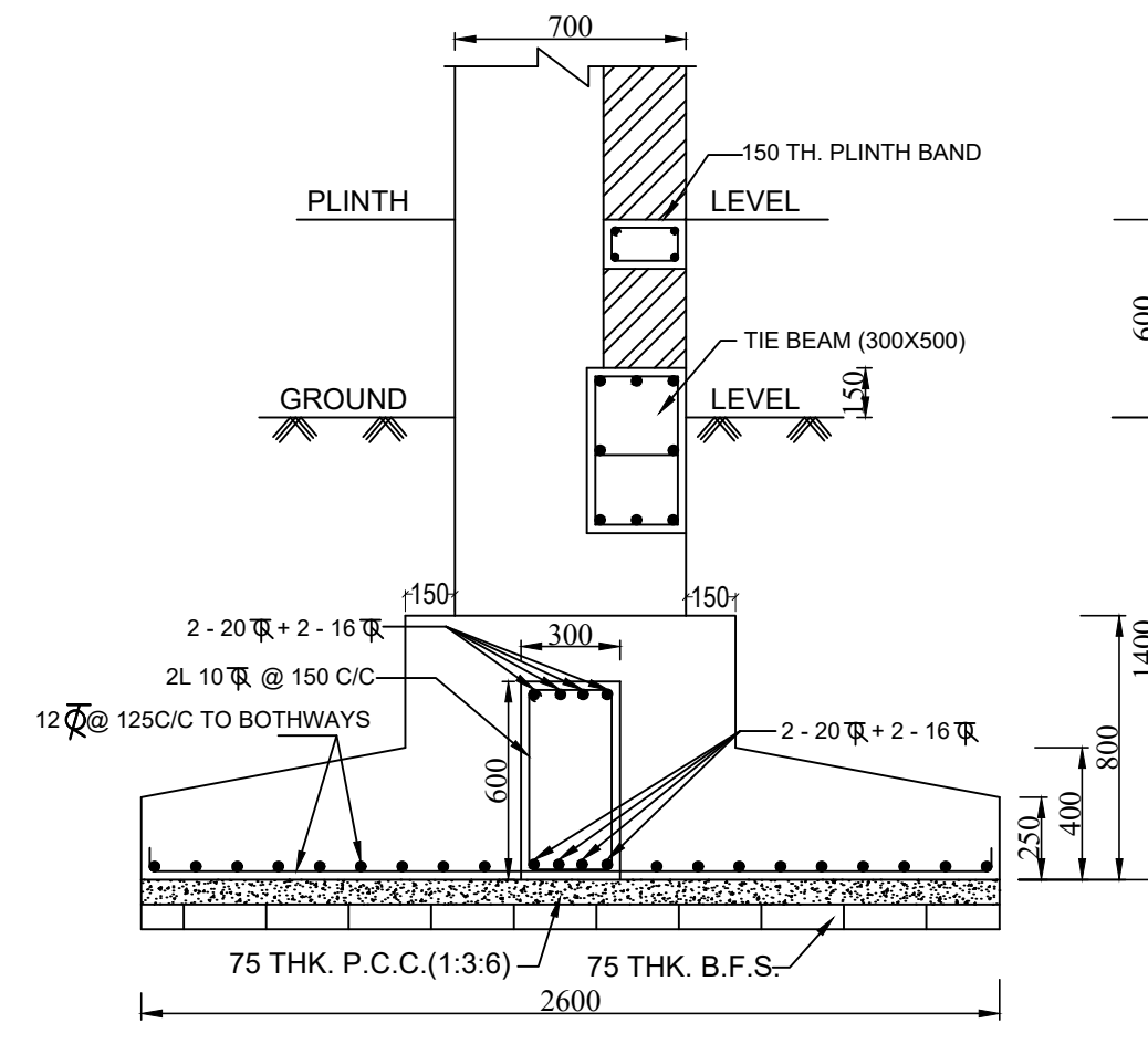
SECTION AT - D-D SCALE-1:25
