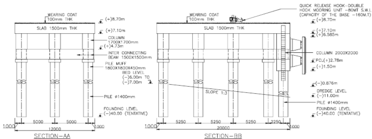
Plan and Section of Berthing Dolphins
