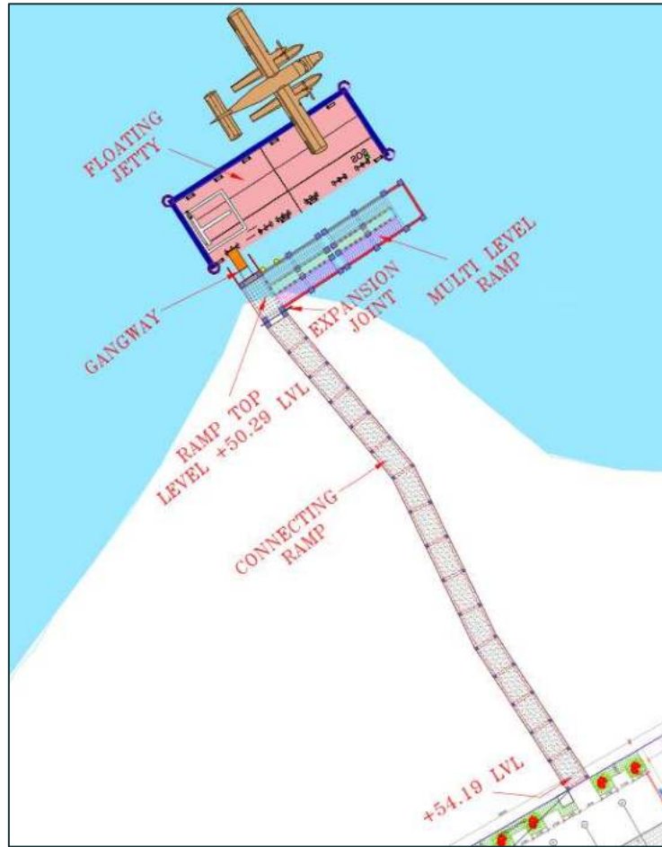
Figure 38 Option-1 Layout
