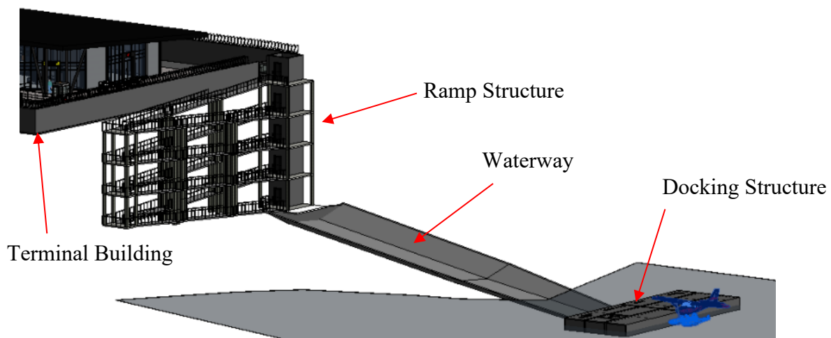
Figure 40 3D Illustration for Option-2
