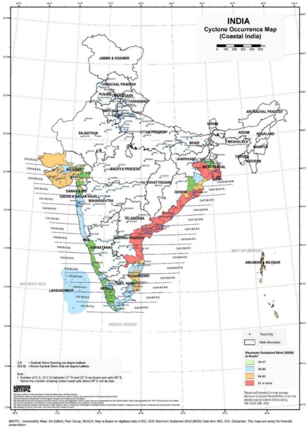
Figure 59 Cyclone Occurrence Map
