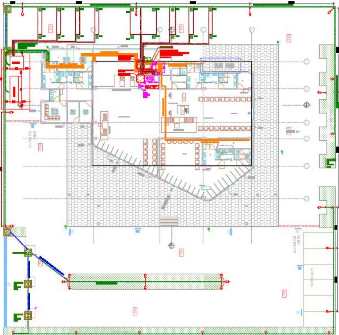
Figure 51 Layout of External Lighting Arrangement
